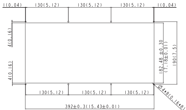
Panel Cutout
