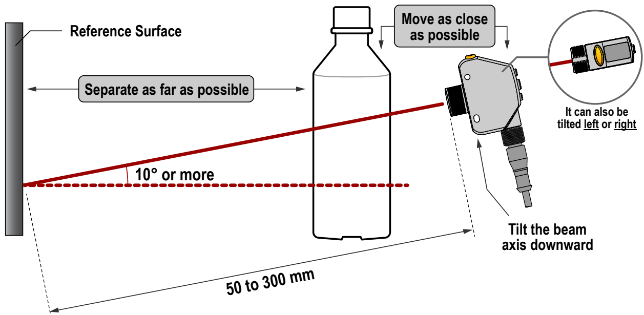
Figure 4. Mounting considerations
